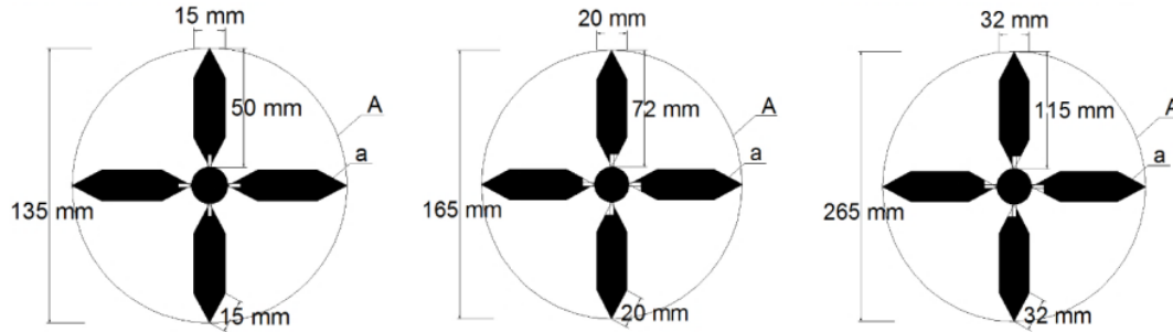
Figure 1. Model of 4-leaf folding anchors for Field Test
