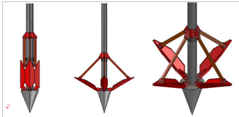
Figure 2. Folding Anchor 3D Model
