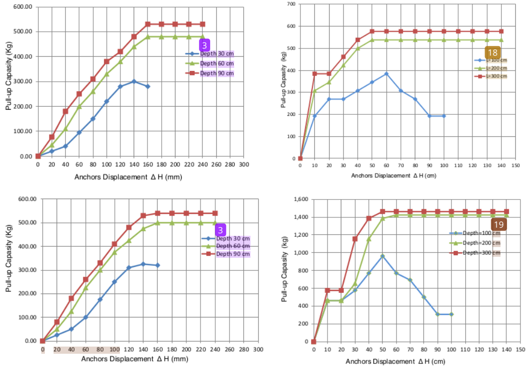
Figure 3. Anchor pull-up capability and depth relationship (Left=Laboratory Test, Right=Field Test)
