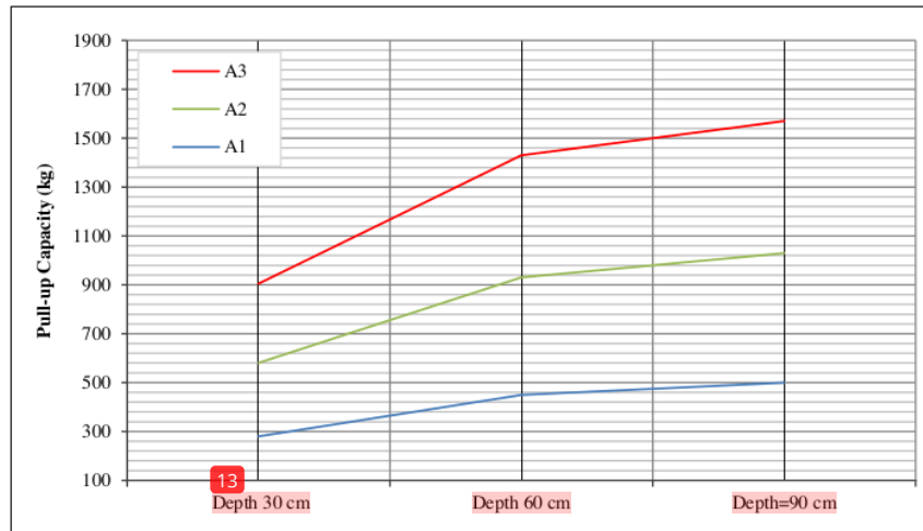
Figure 8. Maximum pull-up capacity against intake depth
